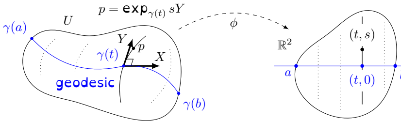
Figure 9.1: Fermi Coordinates
