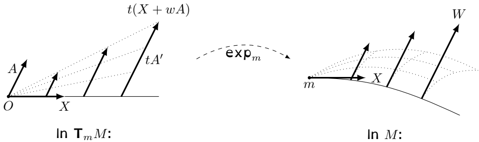
Figure 10.1: Jacobi Field
