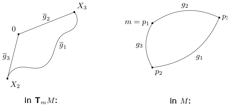
Figure 10.6: Geodesic Triangle
